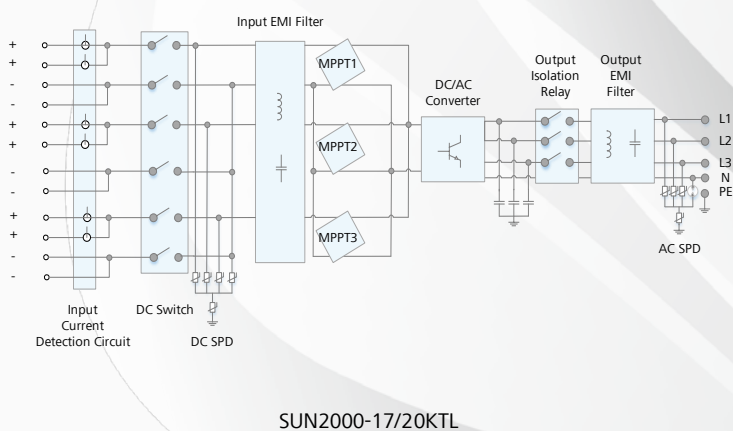
Circuit Diagram
