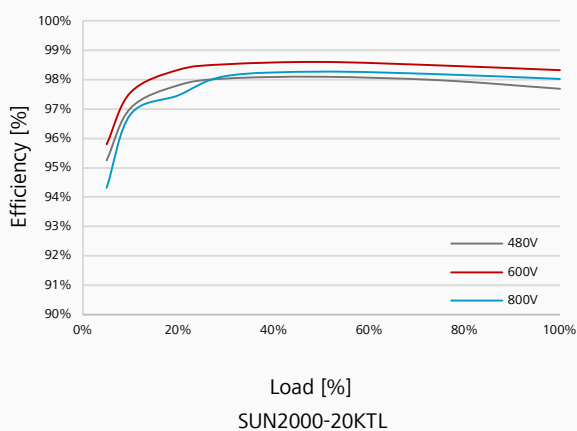
Efficiency Curve
