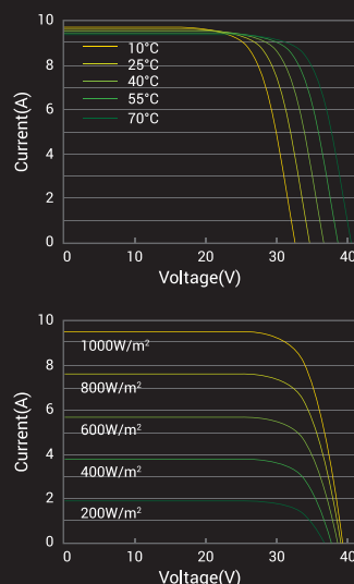
I-V Curve: (A-HCM550)
