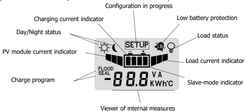
Pic. 4 Display
