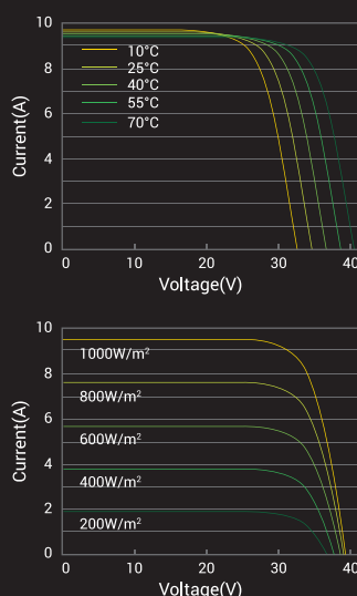
I-V Curve: (A-HCM330)
